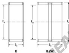
Boundary dimensions for needle roller and cage assemblies
