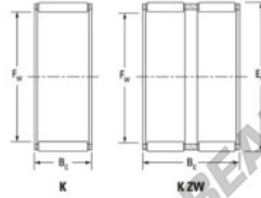
Boundary dimensions for needle roller and cage assemblies
