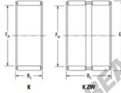
Ball or needle roller and cage assemblies
