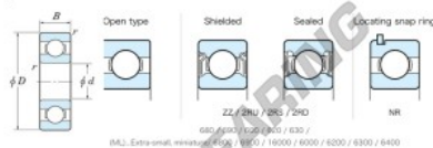
Boundary dimensions
