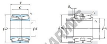
Double-row tapered roller bearings TDO type
